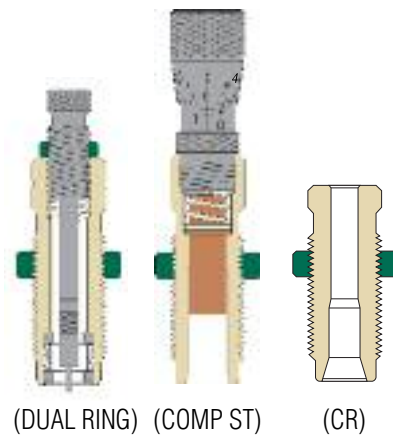
Dual Ring Competition Pro-Series Die Set
